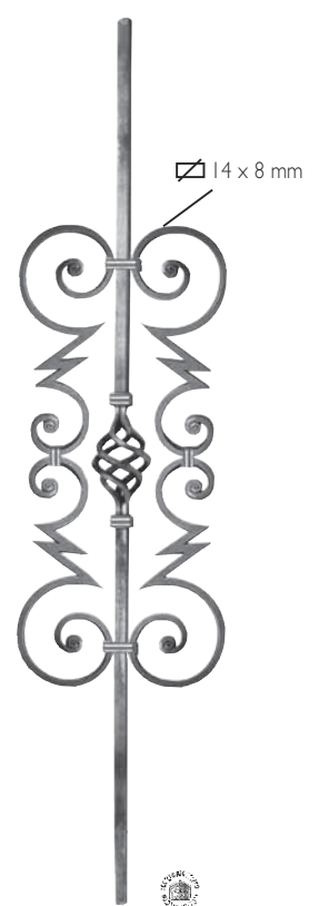
Art. GDI96/3 \Phi 14 x 14 mm H 1000 mm L 215 mm
