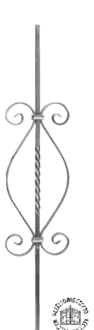
Art. 539/1 \varnothing 12 x 12 mm H 900 mm L 190 mm
