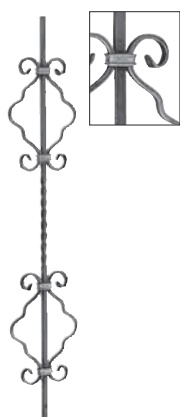
Art. 1127/2 ∅ 12 x 12 mm H 1000 mm L 160 mm
